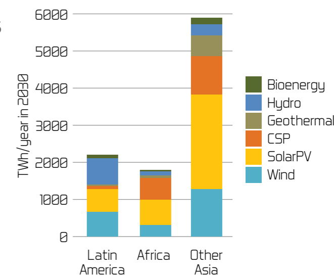
Figure 7 2030 generation by technology under 100% renewables scenario
